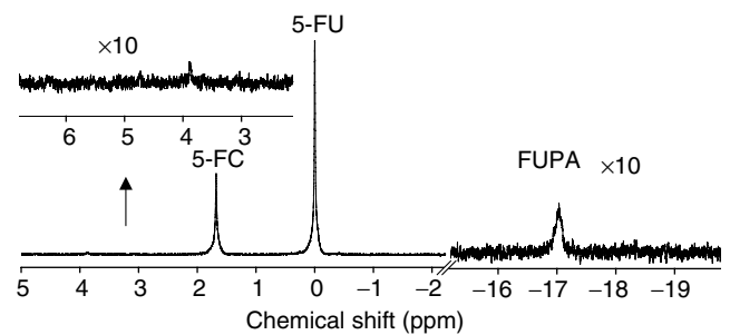
Figure 4 In vitro 19 F MRS spectrum (TR = 2.5 s; NA = 12228; 1 H WALTZ-16 decoupling) of the perchloric acid extract of the whole tumour shown in Figure 2, snap-frozen 2 h 47 min after the in vivo evaluation. A large conversion of 5-FC to 5-FU is visible in agreement with the large delay between in vivo 19 F MRS and span freezing. Only small anabolite ( \sim 4 p.p.m.) and catabolite signals ( \sim -17 p.p.m.) are observed.
