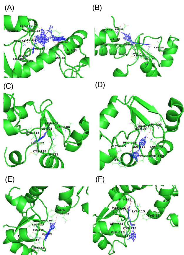
Fig. 3. Interaction profile of E6 with natural ligands carrageenan (A), withaferin A (B), epigallocatechin gallate (C), indole-3-carbinol (D), jaceosidin (E), and curcumin (F) showing interaction of ligands with active site residues of E6 by forming hydrogen bonds, shown in dotted lines.
