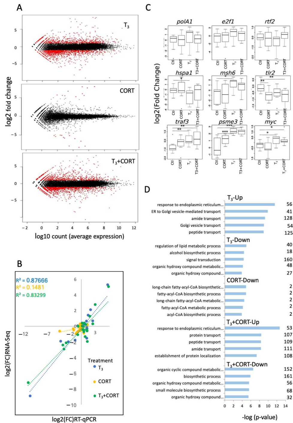
Figure 1. T 3 and CORT treatments induce major changes in gene expression: (A) MA-plots for DE genes following each treatment; (B) validation of the RNA-Seq data by RT-qPCR carried out for 21 genes selected with an average expression level above 100 reads; (C) RT-qPCR validation of gene expression following T 3 , CORT, and T 3 + CORT treatments (statistical significance according to Mann–Whitney test with * p < 0.05 ; ** p < 0.01 ; *** p < 0.001 ); (D) gene ontology analysis of the DE genes.
