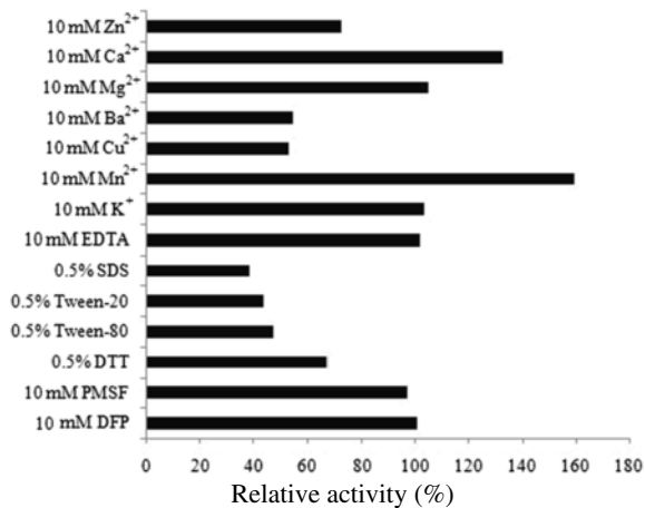
Figure 8 Effect of metal ions, detergents and inhibitors on P. laetus CtpA enzyme stability. Aliquots of the enzyme were incubated with each metal ion (10 mM), detergent (0.5%) and inhibitors (10 mM) at 30°C for 1 h, the residual activity of CtpAp was determined using \beta -casein as the substrate. All determinants were performed in triplicate.
