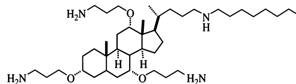
Figure 1. Structure of ceragenin cationic steroid antibiotics (CSA)-13.
