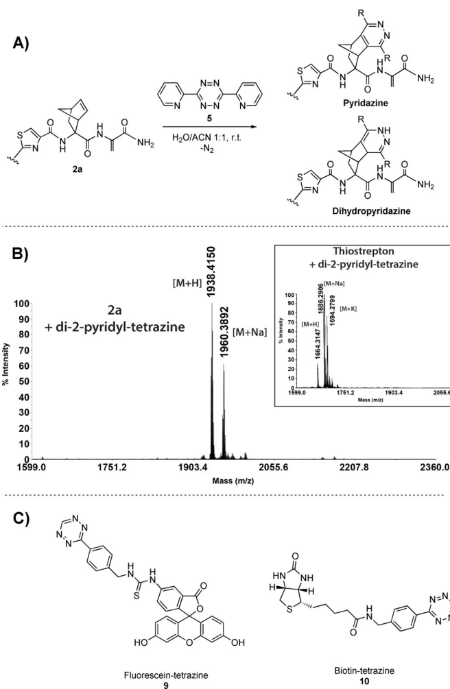
Figure 2. A) IEDDA reaction of norbornene-modified thiostrepton with di-2-pyridyl tetrazine ( 5 ). B) MALDI-TOF MS spectra of IEDDA reaction of di-2-pyridyl tetrazine with 2a and control reaction with unmodified thiostrepton (inset). C) Structures of fluorescein-tetrazine ( 9 ) and biotin-tetrazine ( 10 ).
