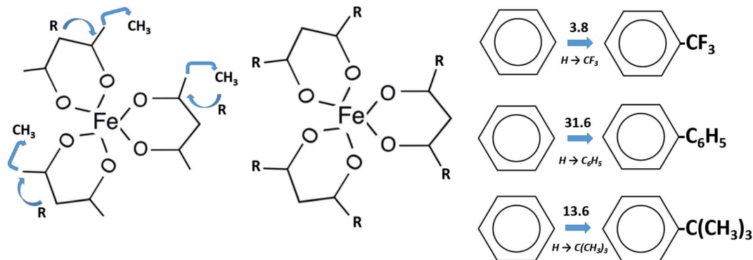
Fig. 10 The road map for estimation of \Delta_1^g H_m^\circ(298.15 \text{ K}) of tris( \beta -diketonato)iron(III) complexes based on the [L]_{(\text{acac})} ligand (the idea – left and the result – middle). Approach for parametrization of contributions H \rightarrow R for the exchange of R substituent on the ligand ring (right). Experimental data involved in the approach are collected in Table S3.†
