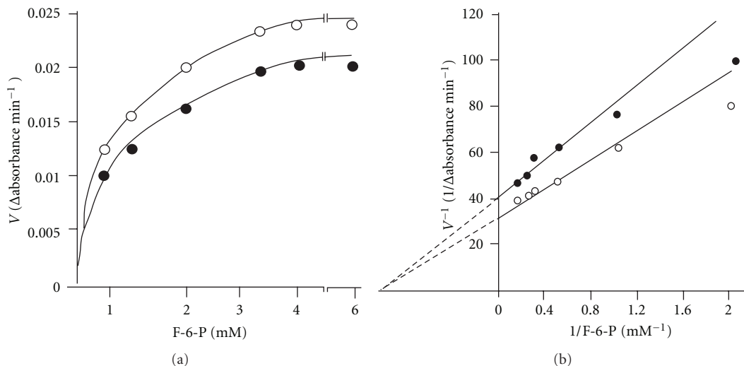
FIGURE 1: Effect of F-6-P concentration on the rate of S. cervi PFK catalyzed reaction. ATP concentration was 50 (○) and 100 (●) \mu\text{M} and \text{Mg}^{2+} concentration was 3.3 mM. Enzyme concentration was 6.6 \mu\text{g}/\text{mL} . Other conditions were same as in standard enzyme assay. (b) Double reciprocal plot of the data of (a). ATP concentrations were 50 (○) and 100 (●) \mu\text{M} .
