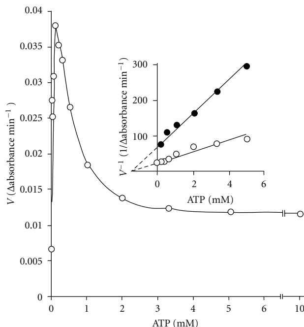
FIGURE 4: Effect of ATP concentration on the rate of PFK catalyzed reaction at fixed concentration of F-6-P and Mg^{2+} (3.3 mM each). Inset shows the plot obtained on assaying the enzyme at variable inhibitory (>0.1 mM) concentration of ATP at two fixed concentrations of F-6-P such as 1.6 (●) and 3.3 (○) mM. Mg^{2+} concentration was constant (3.3 mM). Enzyme concentration was 10 \mu\text{g}/\text{mL} . Other conditions were same as in standard enzyme assay.
