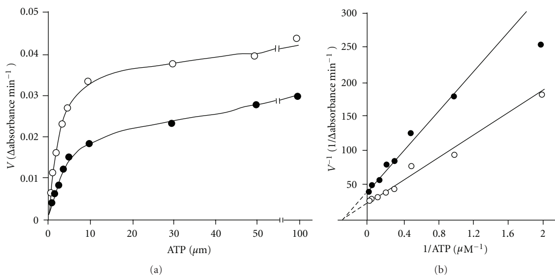
FIGURE 2: Effect of ATP concentration on the rate of PFK catalyzed reaction. F-6-P concentration was 1.6 (○) and 3.3 (●) mM and \text{Mg}^{2+} concentration was 3.3 mM. Enzyme concentration was 10 \mu\text{g}/\text{mL} . Other conditions were same as in standard enzyme assay. (b) Double reciprocal plot of the data of (a). F-6-P concentrations were 1.6 (○) and 3.3 (●) mM.
