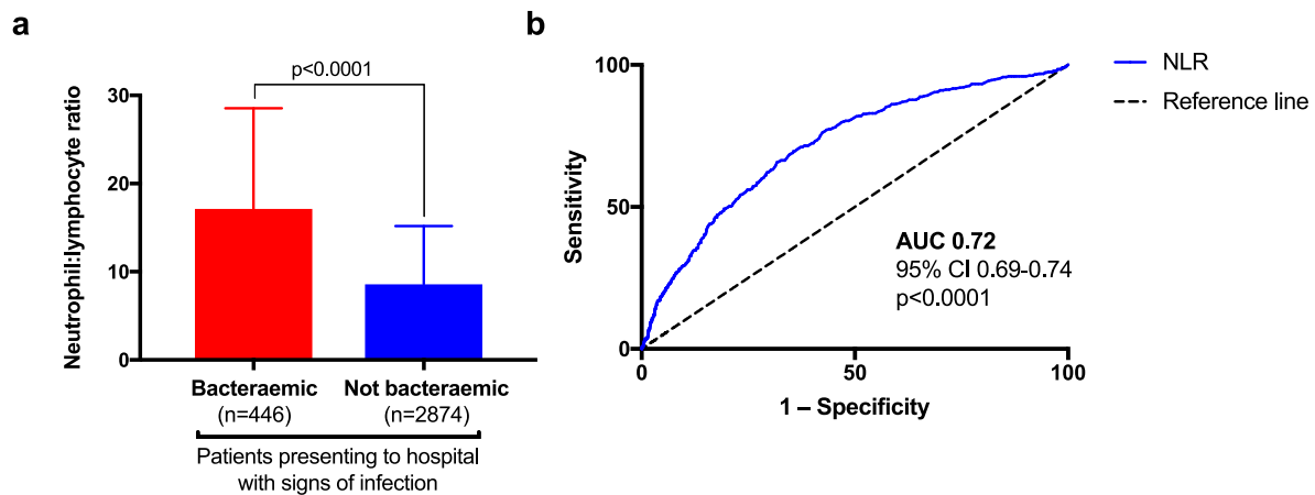
Fig. 3. Meta-analysis results for NLR and bacteraemia. a NLR median and interquartile range derived from meta-analysis of patient-level data for 3320 patients. b Receiver operator characteristic analysis for NLR in predicting presence of bacteraemia in these patients.
