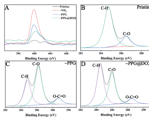
Fig. 2 The fine XPS spectra of material surface modifications. (A) \text{N}_{1s} spectra; (B), (C) and (D) are the \text{C}_{1s} spectra of pristine, \sim\text{PPG} and \sim\text{PPG@DOX} surfaces respectively.
