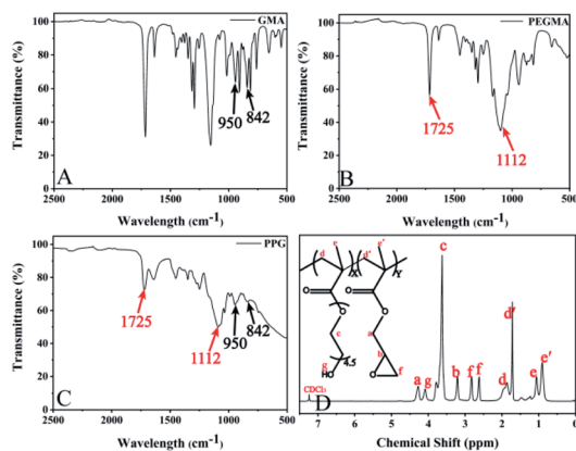
Fig. 1 (A), (B) and (C) are FTIR spectra of GMA, PEGMA and copolymer PPG respectively. (D) ^1\text{H-NMR} spectrum of PPG dissolved in chloroform-d solution.
