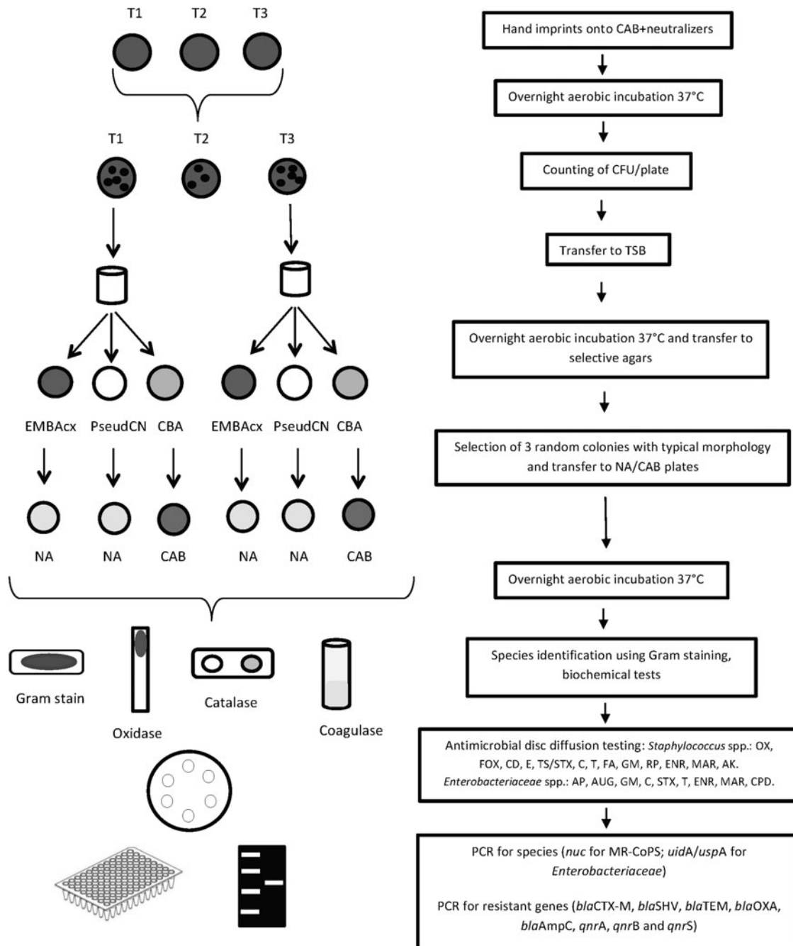
FIG. 1. Schematic view of methods. CAB, Columbia 5% defibrinated horse blood agar; CFU, colony-forming units; TSB, tryptone soy broth; EMBAcx, Eosin Methylene Blue with cefotaxime (1 mg/L); PseudCN, Pseudomonas CN 200 mg/L (Cetrimide and 15 mg/L Sodium Nalidixate); CBA, Chromogenic Brilliance Agar; NA, nutrient agar; OX, oxacillin; FOX, cefoxitin; CD, clindamycin; E, erythromycin; TS/STX, trimethoprim-sulfamethoxazole; C, chloramphenicol; T, tetracycline; FA, fusidic acid; GM, gentamicin; RP, rifampin; ENR, enrofloxacin; MAR, marbofloxacin; AK, amikacin; AP, ampicillin; AUG, amoxicillin clavulanate; CPD, cefpodoxime.
