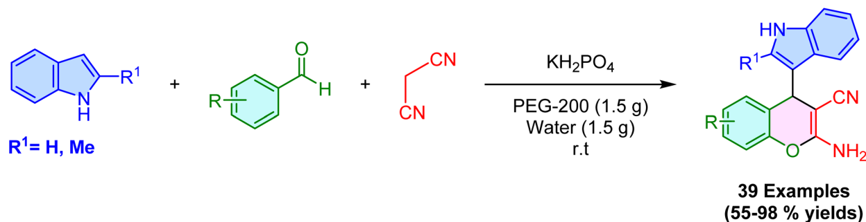
Scheme 3 PEG/KH 2 PO 4 -promoted three-component synthesis of 3-substituted indoles in water.
