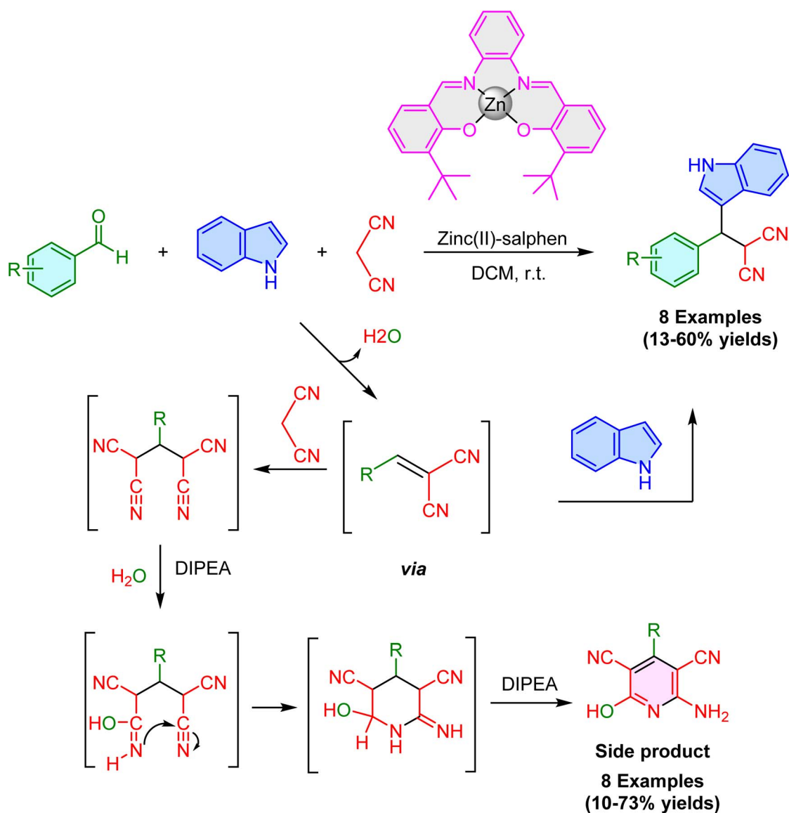
Scheme 46 \text{Zn}(\text{II})(\text{salphen}) -catalyzed synthesis of 3-substituted indoles.
