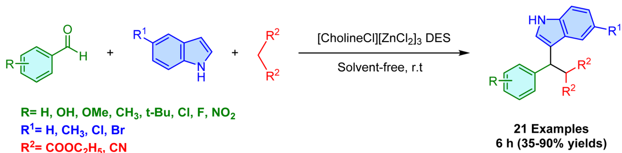
Scheme 31 [cholineCl][ZnCl 2 ] 3 DES-catalyzed solvent-free synthesis of 3-substituted indoles.
