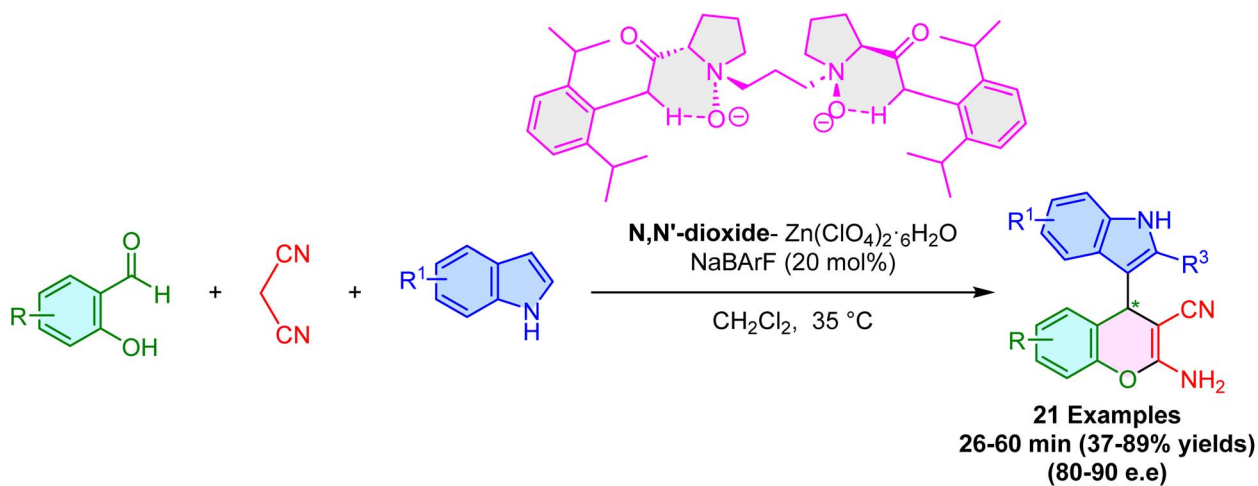
Scheme 45 N,N' -Dioxide \text{Zn}(\text{II}) complex-catalyzed enantioselective one-pot synthesis of 2-amino-4-(indol-3-yl)-4H-chromenes.
