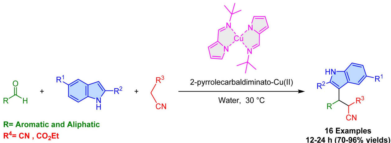
Scheme 41 2-Pyrrolinecarbaldehyde–Cu(II) complex-catalyzed aqueous synthesis of 3-substituted indoles.
