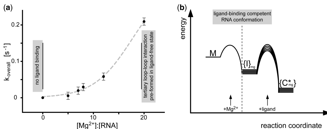
Figure 5. Mg^{2+} dependence of the ligand-induced Gsw^{loop} folding; (a) overall time constant k_{overall} [s -1 ] of ligand-induced RNA folding process as a function of [Mg^{2+}]:[RNA] ratio (the error is given from replica measurement at [Mg^{2+}]:[RNA] \sim 7:1 ; additional data at higher [Mg^{2+}]:[RNA] ratios >20:1 could not be obtained due to the limited time-resolution of the NMR measurements; gray dashed line: sigmoidal fit; the choice of the fitting function was motivated by assuming that k_{overall} [s -1 ] approaches saturation at an [RNA]:[Mg^{2+}] ratio of 1:20); (b) free activation energies of the Mg^{2+} - and/or ligand-induced conformational transitions are schematically depicted. In the free G37A/C61U-mutant (M, absence of Mg^{2+} ), secondary structure elements but neither the loop-loop interaction nor the ligand-binding region are pre-formed and Gsw^{loop} cannot bind ligand (28). Through variation of the [RNA]:[Mg^{2+}] ratio, the ligand-binding capability can be restored ( \{I\}_{mg} ) as well as formation of the tertiary loop-loop interaction at high Mg^{2+} concentrations ( [RNA]:[Mg^{2+}] > 1:18 ). In the schematic diagram, this observation leads to a conformational RNA ensemble, whose dynamic and structural properties are Mg^{2+} dependent (signified by \{\} ). The addition of Mg^{2+} leads to a rapid RNA conformational change. The derivation is based on the experimental finding that the Mg^{2+} -induced conformational transition, monitored for Gsw^{loop} at an [RNA]:[Mg^{2+}] ratio <1:18 ( M \rightarrow \{I\}_{mg} ), is faster than \sim 8 – 10 s. The conformational transitions induced by Mg^{2+} are very fast and associated with energetic barriers that are small compared to the barriers associated with ligand binding. The kinetics of ligand binding ( \{I\}_{mg} \rightarrow \{C^*\}_{mg} ) strongly dependent on the [RNA]:[Mg^{2+}] ratio. The variation in kinetic rate constants from the [Mg^{2+}] concentration implies Mg^{2+} -dependent differences of the free activation energy.
