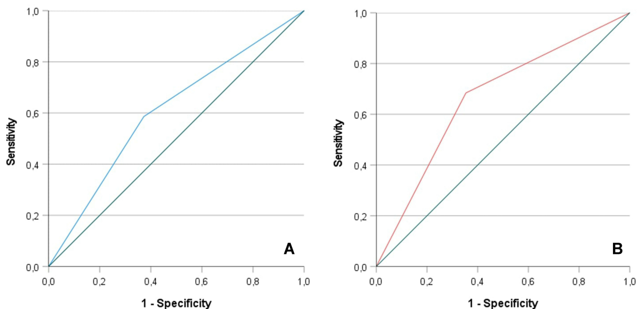
Figure 1 Receiver-operating characteristic (ROC) curves showing the discrimination performance of NLR cut off values in the derivation (IA) and validation (IB) cohort.
