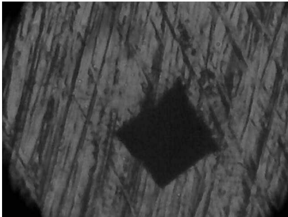
Fig. 1. Indentation made with the Vickers hardness machine
