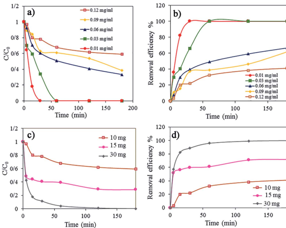
Fig. 8 (a) Effect of contact time and dye concentration on the adsorption of AR1 dye on 3D \text{rGO@Fe}_3\text{O}_4 (temp. = rt, pH = neutral, and adsorbent dosage: 10 mg). (b) Effect of dye concentration on the removal efficiency% of AR1 dye. (c) Effect of adsorbent dosage on adsorption of AR1 ( 0.12 \text{ mg mL}^{-1} ). (d) Effect of adsorbent dosage on removal efficiency% of AR1 ( 0.12 \text{ mg mL}^{-1} ).
