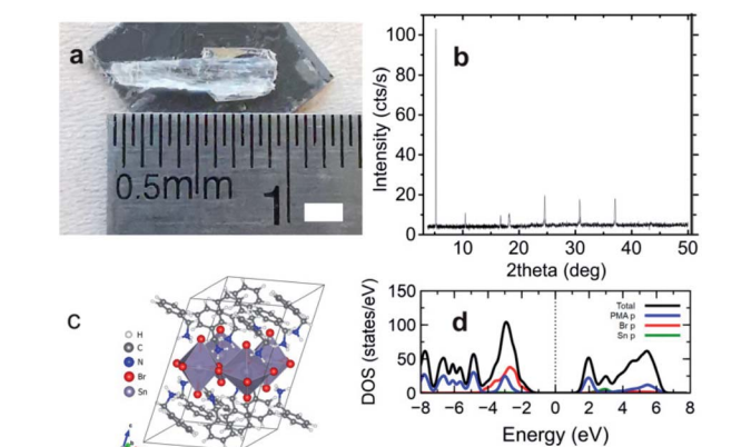
Fig. 1 Appearance and structure of (\text{C}_6\text{H}_5\text{CH}_2\text{NH}_3)_2\text{SnBr}_4 . (a) A photograph of a large crystal with a scale bar of 2 mm. (b) X-ray diffraction pattern. (c) Crystal structure representation. (d) Total (black) and projected (color) density of states (DOS). Blue, green, and red lines represent (\text{C}_6\text{H}_5\text{CH}_2\text{NH}_3) s and p, Sn p, and Br p orbitals, respectively.
