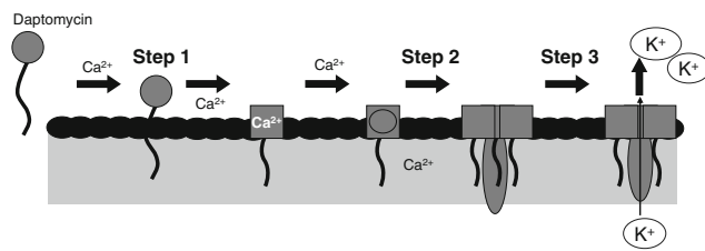
Fig. 1 Mechanism of action of daptomycin [48]. Reprinted with permission. Step 1 calcium-dependent binding and insertion of the lipophilic tail into Gram-positive cytoplasmic membrane. Step 2 oligomerization and channel formation occur. Step 3 ion leakage and collapse of organism lead to cell death
