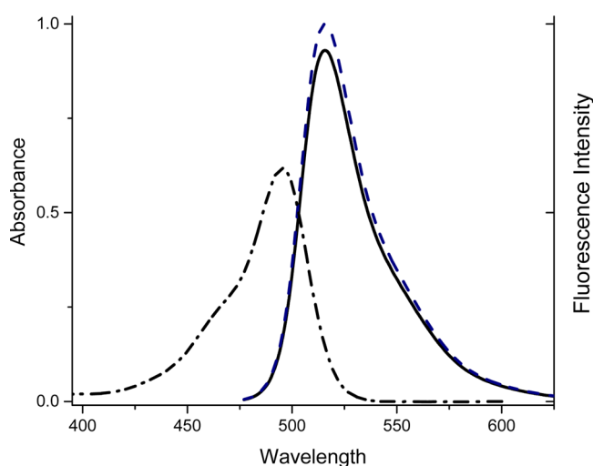
Figure 3. Absorption (dash-dotted line) and emission spectra (solid line) of 11 \mu\text{M} PBS solution of BSA-fluorescein conjugate ( 10 ) and emission spectrum of a 11 \mu\text{M} PBS solution of fluorescein (dotted line).
