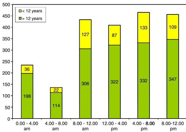
Fig. 2 Temporal arrival of patients ( n=2,134 )
