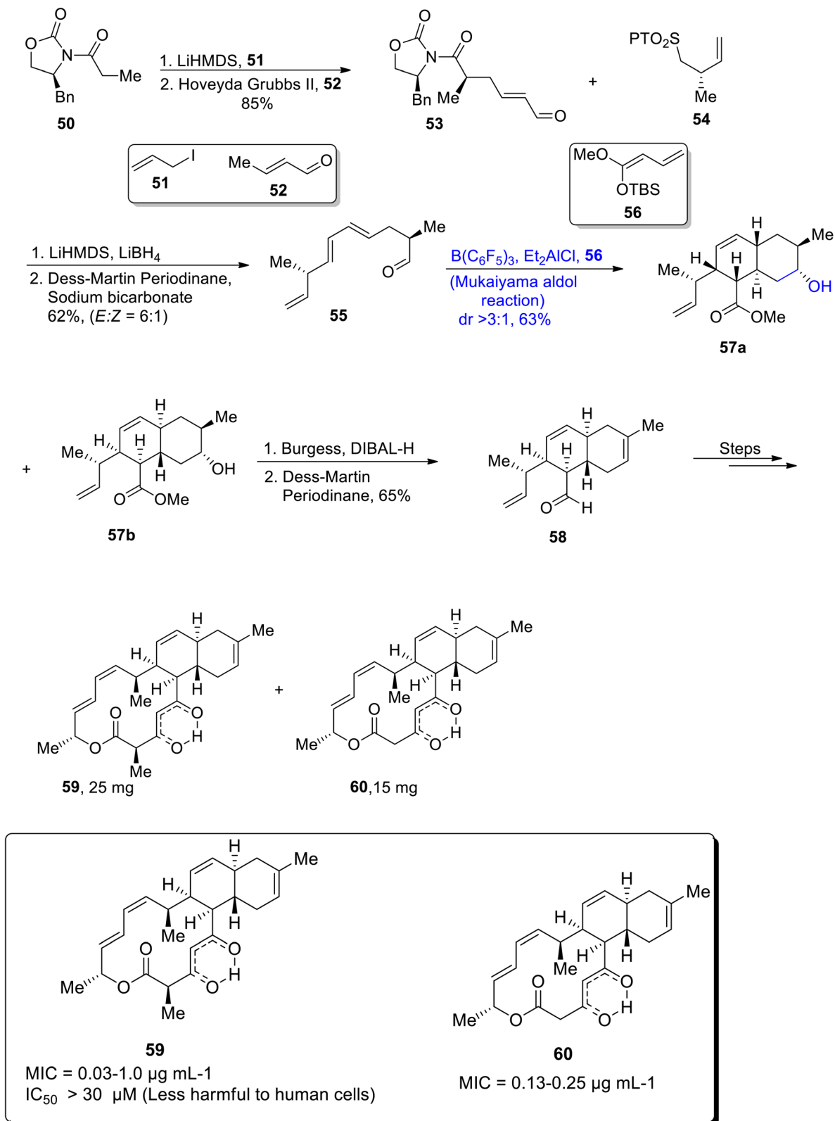
Scheme 7 Synthesis of anthracimycin 59 and anthracimycin B 60 .
