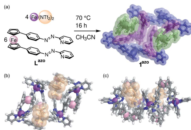
Fig. 2 Crystal structure of \mathbf{1}^{\text{azo}} . (a) \text{L}^{\text{azo}} assembled with \text{Fe}^{\text{II}} ions to form \mathbf{1}^{\text{azo}} via guest templation. Crystal structure (right) is viewed down the C_2 axis with each magnetically-unique ligand displayed in a different color. (b) With two \text{Tf}_2\text{N}^- anions (depicted in beige) binding in distinct pockets (c) View perpendicular to the C_2 axis, with two \text{Tf}_2\text{N}^- anions. The remaining anions, disorder and solvent are not shown for clarity.
