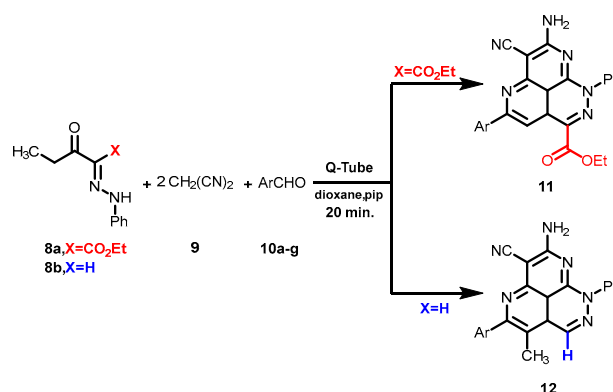
Scheme 2. Novel synthesis of the tricyclic system 11 by reacting ethyl-3-oxo-2-(2-phenylhydrazono)pentanoate ( 8a ) with malononitrile ( 9 ) and aromatic aldehyde derivatives 10 in a Q-Tube.
