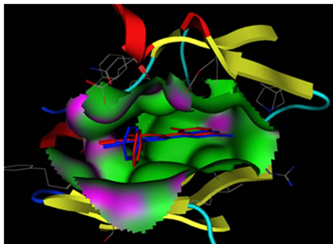
Fig. 4. 3D representation of the best pose of co-crystallized inhibitor (blue color) docked into the binding site and superimposed on co-crystallized inhibitor (red color) in the crystal structure of PIM-1 kinase was also shown (PDB ID: 20BJ).
