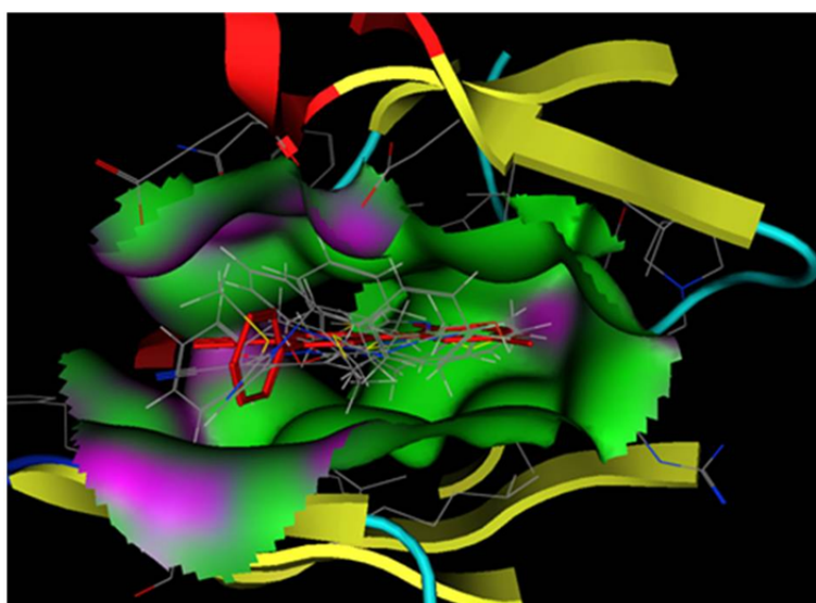
Fig. 5. Seven docked compounds superimposed in binding cavity of PIM-1 kinase. Compounds represent as line and colored by atom. Co-crystallized inhibitor is also shown as stick and red. Green hydrophobic, violet hydrogen bond and blue as middle polar represent electrostatic map of binding cavity.
