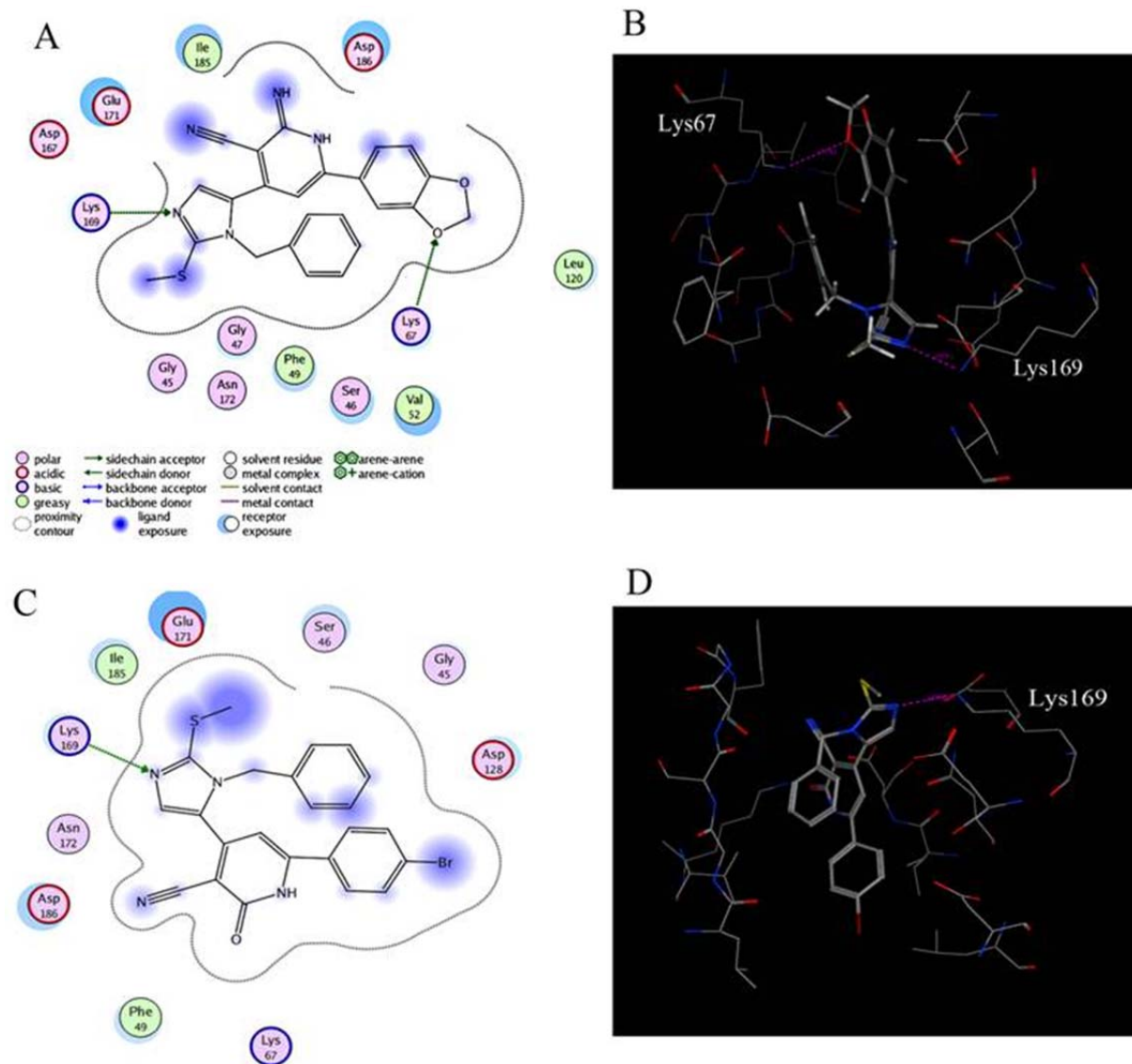
Fig. 6. 2D graphs of interactions between compounds, (A) Ic , (C) IIa , and PIM-1 kinase (PDB ID: 20bj). Graphs are made using MOE software. In this plots hydrophobic/aromatic residues are colored in green, whereas polar amino acids in magenta. H bonds are shown as green dotted lines. The active site contour is also shown. Part B and D demonstrate 3D position of compound Ic and IIa (respectively) in active site of enzyme, hydrogen bonds are also shown as violet dotted lines.
