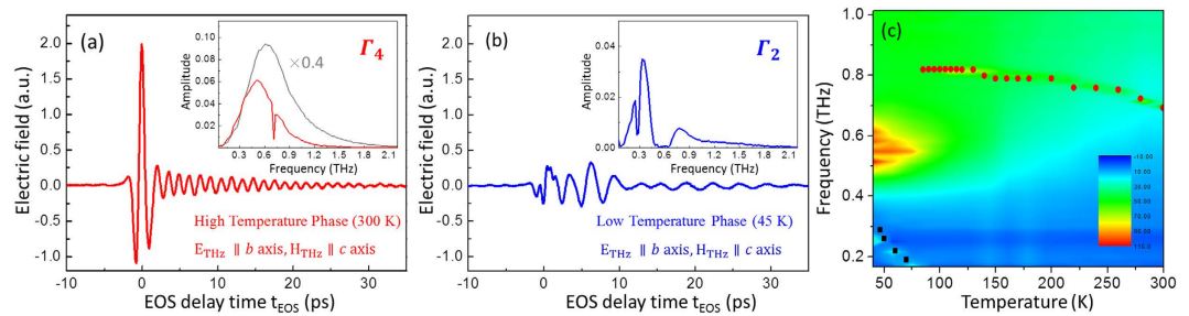
Figure 1. (a) The electric field of the THz wave passing through a -cut TmFeO 3 single crystal at (a) high (300 K) and (b) low temperature phase (45 K) with E_{\text{THz}} \parallel b axis, H_{\text{THz}} \parallel c axis. Inset: the Fourier spectral amplitudes of the THz electric fields from the electro-optic sampling signals. The black curve in the inset of (a) is the THz spectrum without sample (dry nitrogen) (c) The amplitude mapping of absorption spectrum of the a -cut TmFeO 3 crystal as a function temperature. The resonant frequencies of FM (square symbols) and AFM (circular symbols) modes are shown as functions of temperature.
