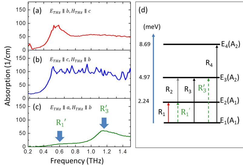
Figure 4. Absorption coefficient of TmFeO 3 at 60 K with different excitation geometries (a) H_{THz} || c, E_{THz} || b in a -cut crystal, (b) H_{THz} || b, E_{THz} || c in a -cut crystal, and (c) H_{THz} || b, E_{THz} || a in c -cut crystal. (d) Energy diagram of ground multiplets of Tm ions.
