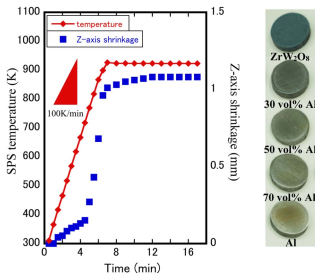
Fig. 1 Z-axis linear shrinkage curve of Al 50 vol% \text{ZrW}_2\text{O}_8/\text{Al} composite and optical photos of \text{ZrW}_2\text{O}_8/\text{Al} composites.
