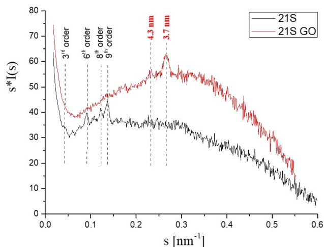
Figure 5 Comparison of SAXS curves ( s [scattering vector] = 2\sin(\theta)/\lambda ) of burnt-burnt human skin (21S) and burnt human skin incubated in the presence of graphene oxide (21S GO).
