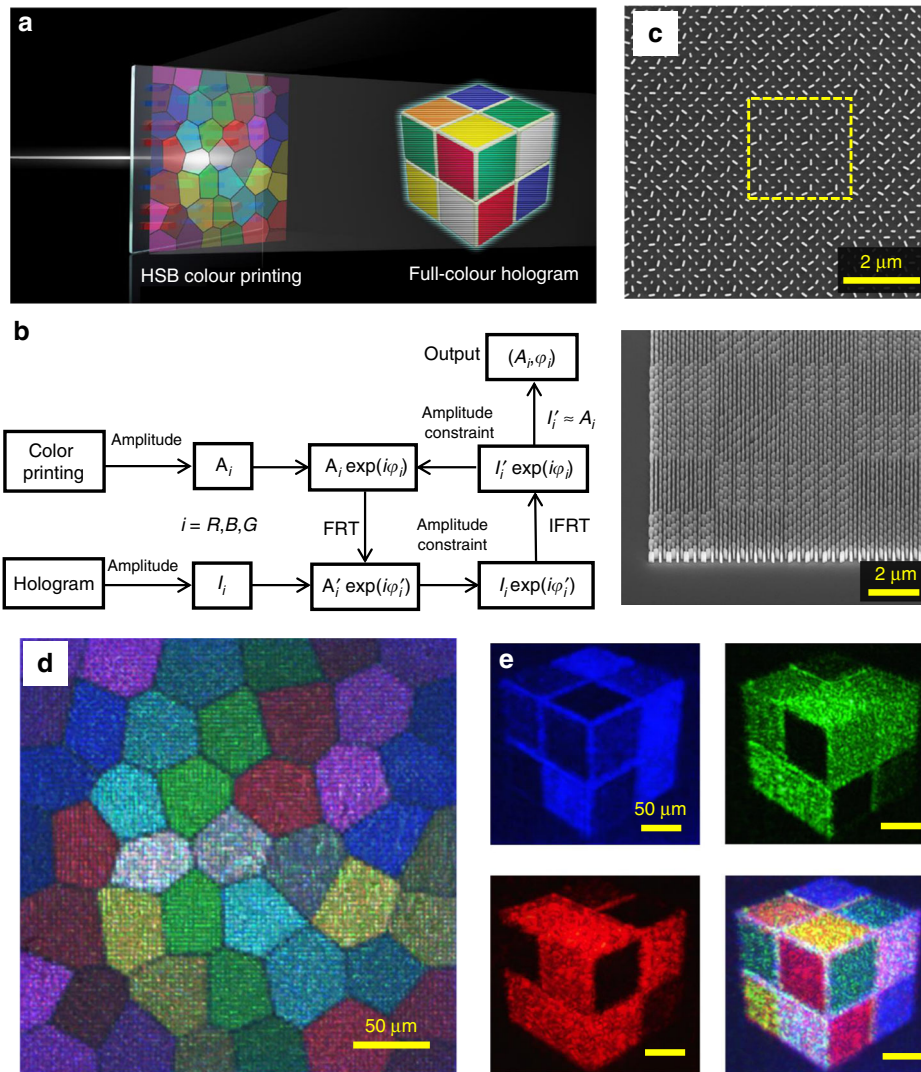
Fig. 5 Integration of HSB colour printing and full-colour hologram. a Schematic of the metasurface for the integration of HSB colour printing and the full-colour hologram image. The hologram plane is designed at 1075 \mu\text{m} above the colour printing image. b Flow chart of the metasurface design for the integration of colour printing and holography. A_i and I_i are the intensities of the three RGB components ( i = R, G, B ) in the colour printing image and hologram, respectively. FRT and IFRT represent the Fresnel transformation and inverse Fresnel transformation, respectively. c Top (upper) and tilted ( 45^\circ , lower) views of the fabricated metasurface. The dashed yellow line indicates an enlarged pixel, which consists of 4 \times 4 RGB units. d Measured optical printing images. e Measured hologram images illuminated by lasers with a wavelength at only 473 nm (top left), 532 nm (top right), 633 nm (bottom left) and all three simultaneously (bottom right)
