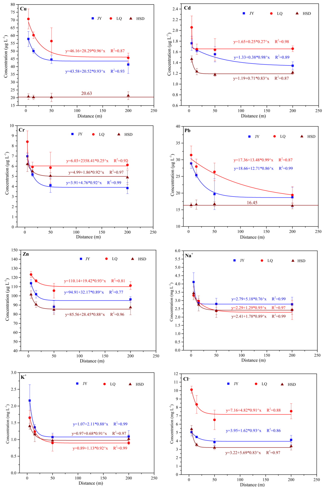
Figure 3. Regression curves of highway-related pollutants concentrations in groundwater in turfy swamp.
