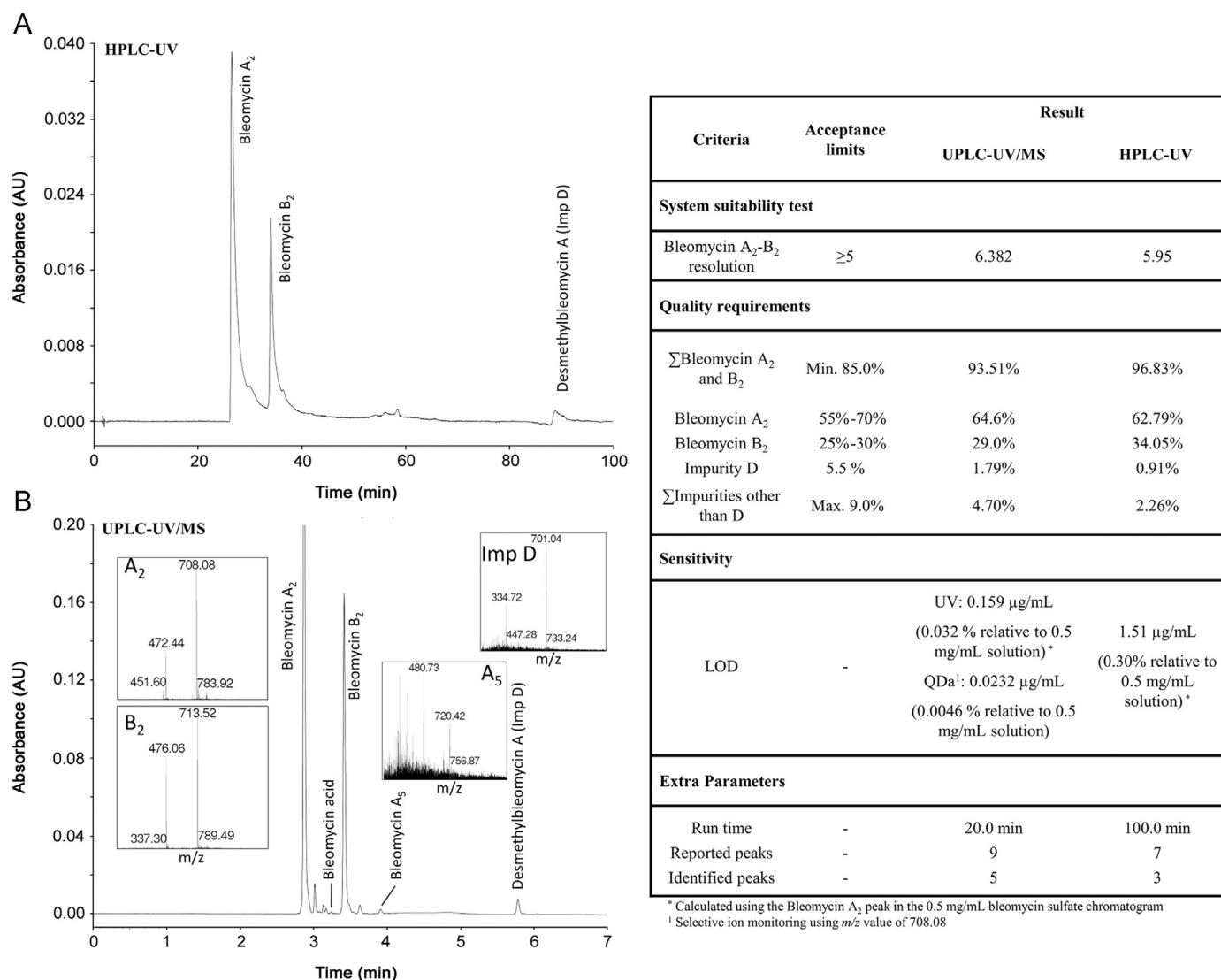
Fig. 1. Bleomycin sulfate (0.5 mg/mL) HPLC-UV (A) and UPLC-UV/MS (B) analysis with identification of major compounds and method comparison. The MS 1 spectra of the main compounds bleomycin A 2 and B 2 , as well as impurities bleomycin A 5 and demethylbleomycin A 2 , are given.
