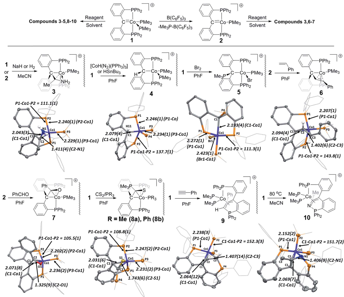
Fig. 5 Products from reactivity of 1 and 2 with various small molecules. Phenyl and methyl hydrogen atoms, and [BAR 4 ] - anions omitted for simplification. Thermal ellipsoids shown at 50%, selected bond distances (Å) and angles (°) displayed.
