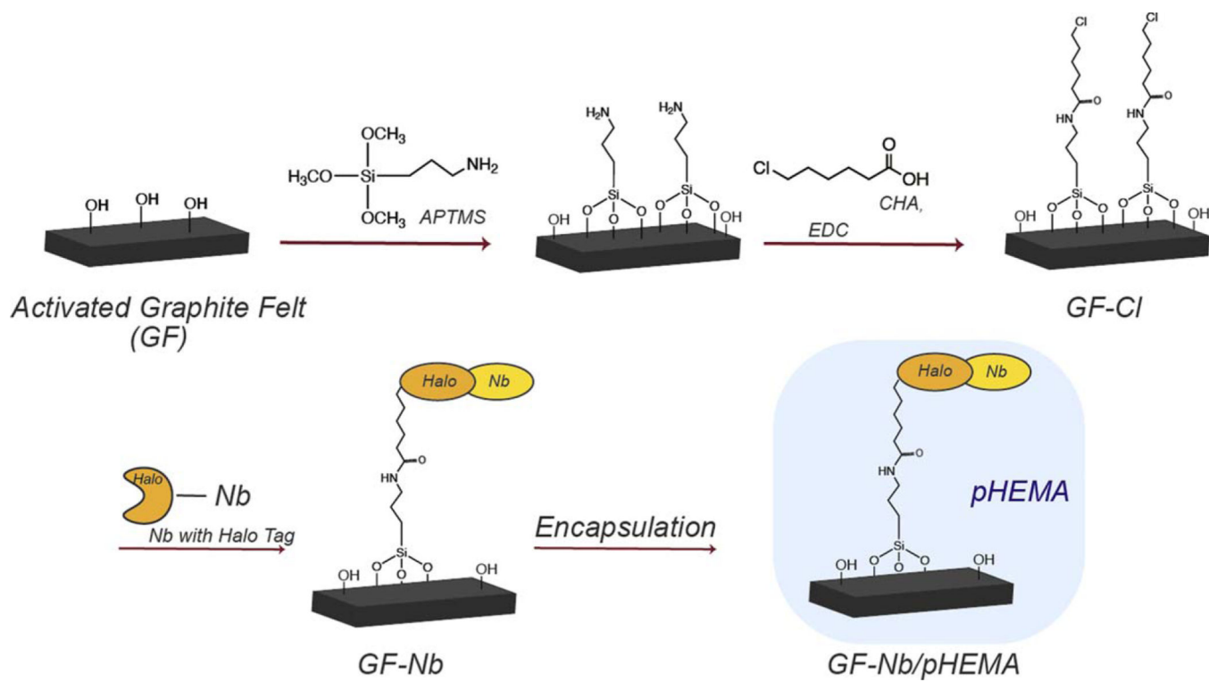
Figure 1. Summary of the process to create nanobody-decorated, encapsulated graphite felt working electrodes.
