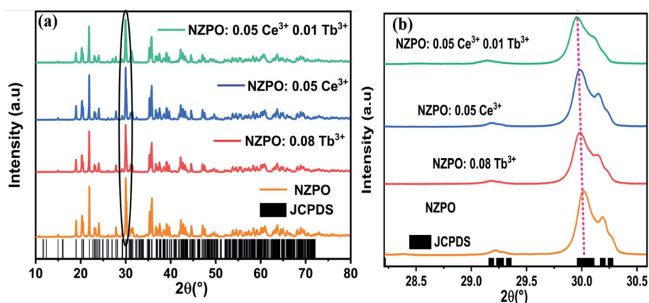
Fig. 1 (a) Powder XRD patterns of NZPO, \text{NZPO}:0.05\text{Ce}^{3+} , \text{NZPO}:0.08\text{Tb}^{3+} and \text{NZPO}:0.05\text{Ce}^{3+}/0.01\text{Tb}^{3+} (b) magnified XRD patterns in the region between 28.30 and 30.60^\circ .
