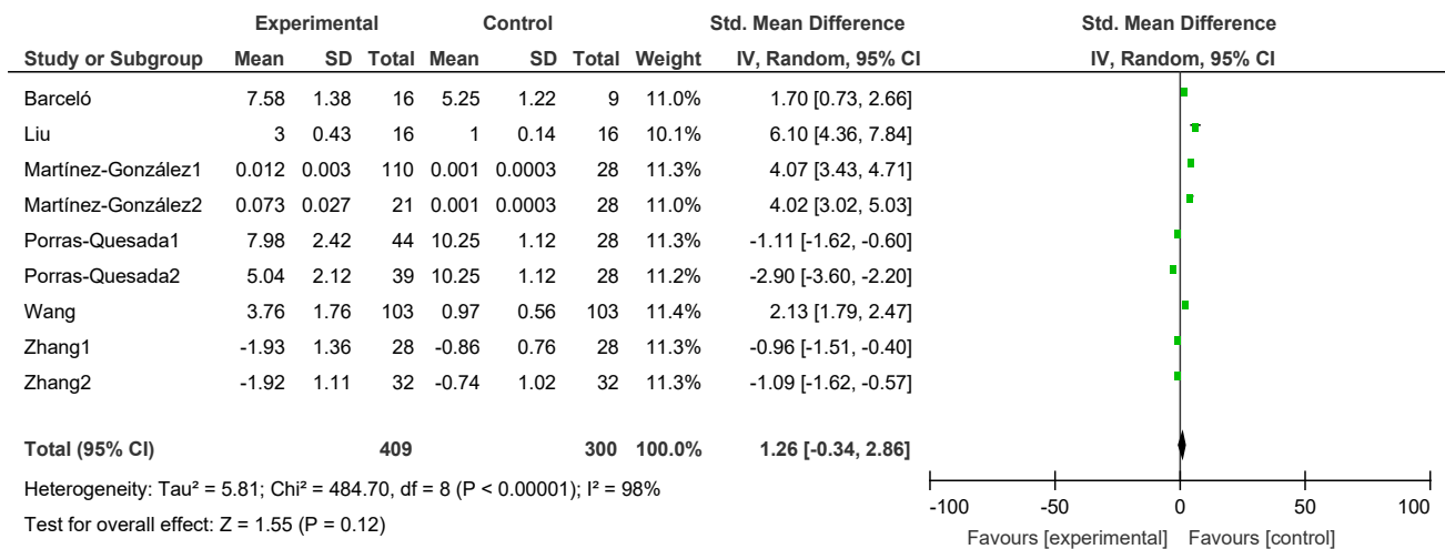
Fig. 2: Random-effects SMD for the association of miR-93 expression level and PCa
