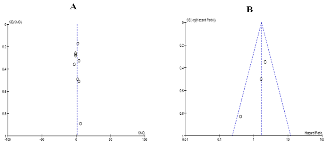
Fig. 4: Funnel plot of A) standardized mean difference, B) hazard ratio
