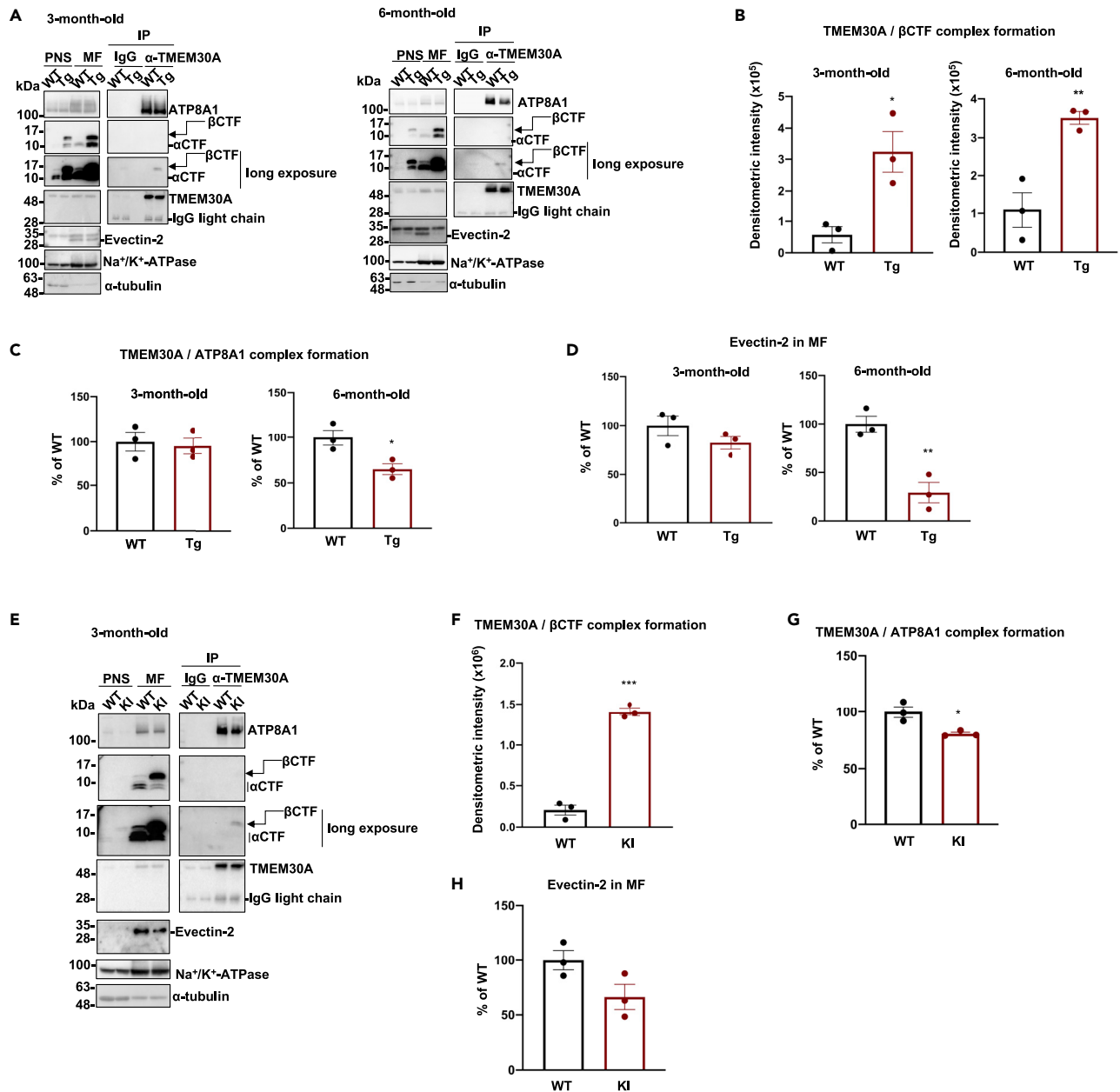
Figure 4. TMEM30A interacts with \beta CTF in AD model mice, which follows by lipid flippase dysfunction
