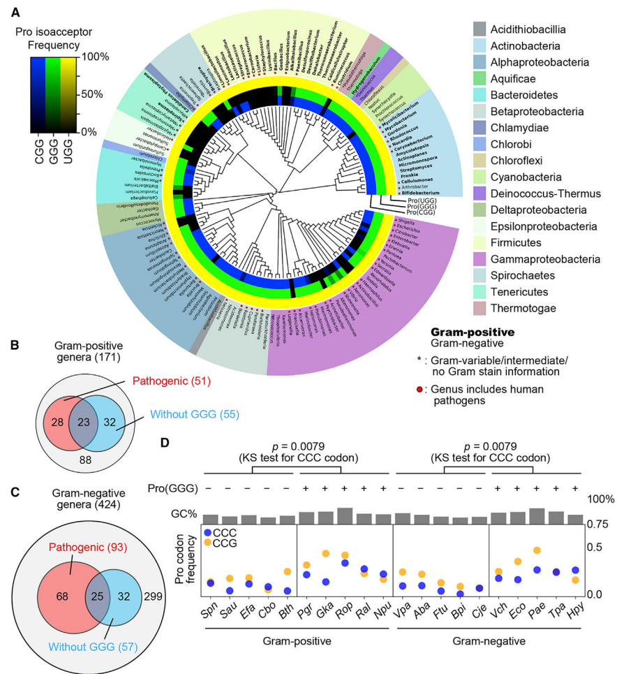
Figure 6. Absence of Pro(GGG) from some bacterial species
