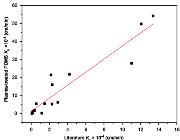
Fig. 5. Relationship between experimental K_p values (plasma-treated membrane) and literature K_p values ( R^2 = 0.88 ).
