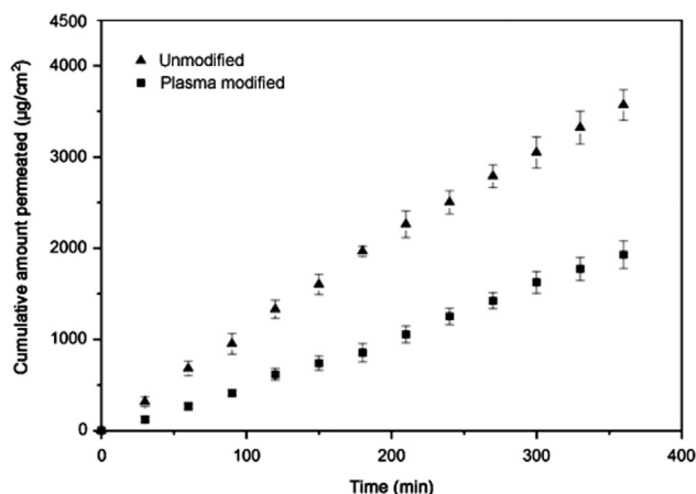
Fig. 1. Cumulative amount permeated for benzoic acid using ( \blacktriangle ) unmodified silicone membrane and ( \blacksquare ) plasma surface-treated silicone membrane ( n=3 , \pm SD).
