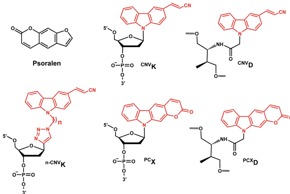
Fig. 13 Carbazole derivatives. Both ^{CNVK} and ^{PCX} carbazole derivatives are inspired from psoralen. Either the vinyl in ^{CNVK} , ^{CNVD} , ^{n-CNVK} or the pyrene in ^{PCX} , and ^{PCXD} undergo reversible [2 + 2] photoreaction.
