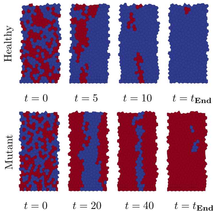
Fig. 6 Mutant cells invade the crypt. Top) probability of mutant cells taking over the crypt as a function of initial proportion of mutated cells, for the VL and Tan models as the mutation parameter \gamma is varied. results are presented for \gamma = 0 (red), 0.5, 0.75, 0.9, and 1 (blue) and the arrow is in the direction of increasing \gamma Bottom) Snapshots of 2 simulations with 50% mutated cells. In the top simulation healthy cells happen to out compete the mutant cells, in the bottom simulation mutant cells win. Note, specific simulations were chosen to illustrate the conversion to homogeneous crypts
