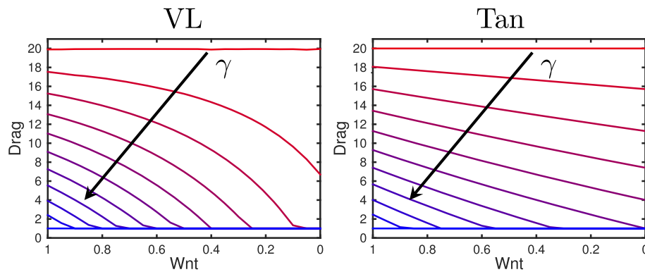
Fig. 3 Drag functions. Drag as a function of the level of complex in the cytosol/membrane ( C_A in the VL model and N_C in the Tan model). The lower \gamma , the higher the drag. I.e. for mutant cells the amount of complex in the cytosol/membrane increases, as seen in Fig. 8, and we assume that this increases the drag. Also when the Wnt signal is higher, the drag will be higher for \gamma \neq 0 (as the amount of complex is higher). Arrows are drawn in the direction of increasing \gamma . The cases are shown for \gamma = 0 - 1 in increments of 0.1 ( \gamma = 0 is red, \gamma = 1 is blue)
