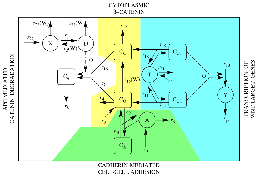
(a) VL
