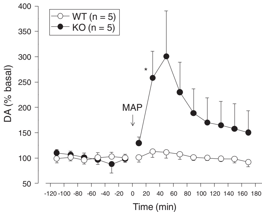
Figure 8 In vivo microdialysis analysis of mGluR3 KO mice. Methamphetamine (MAP) induced the release of dopamine in the nucleus accumbens of mGluR3 KO mice. The extracellular dopamine levels of WT and KO mice were determined by in vivo microdialysis and HPLC. After the collection of basal fractions, MAP (2 mg/kg, i.p) was administered at time 0. Data are given as mean ( \pm SEM) for the indicated number of mice. Repeated-measures analysis of variance revealed a genotype effect of F_{1,88} = 61.9 ( p < 0.001 ), a time effect of F_{8,82} = 3.74 ( p < 0.01 ), and a genotype \times time effect of F_{8,82} = 2.49 ( p = 0.02 ). * p < 0.05 (Bonferroni post-hoc test).
