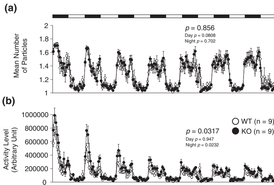
Figure 3 Twenty-four hour home cage monitoring test. Two animals of the same genotype were put in a cage, and their activity was monitored over ~7.5-day period. (a) Social interaction activity was represented as the number of particles in the image of the cage as viewed by automatic detection. When the animals were separated, two particles were seen, and when they were together, only one was observed. Social interaction in their home cage was not obviously different between genotypes. (b) The locomotor activity of KO mice was significantly greater than that of WT mice. Each dot indicates the mean per hour. The p -values indicate a genotype effect in the two-way repeated measures ANOVA. Data are given as mean ( \pm SEM).
