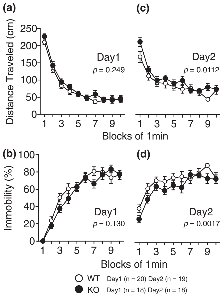
Figure 5 Porsolt forced swim test. Distance traveled ( a, c ) and immobility ( b, d ) were recorded in the Porsolt forced swim test for 2 trials. The p -values indicate a genotype effect in the two-way repeated measures ANOVA. Data are given as mean ( \pm SEM).
