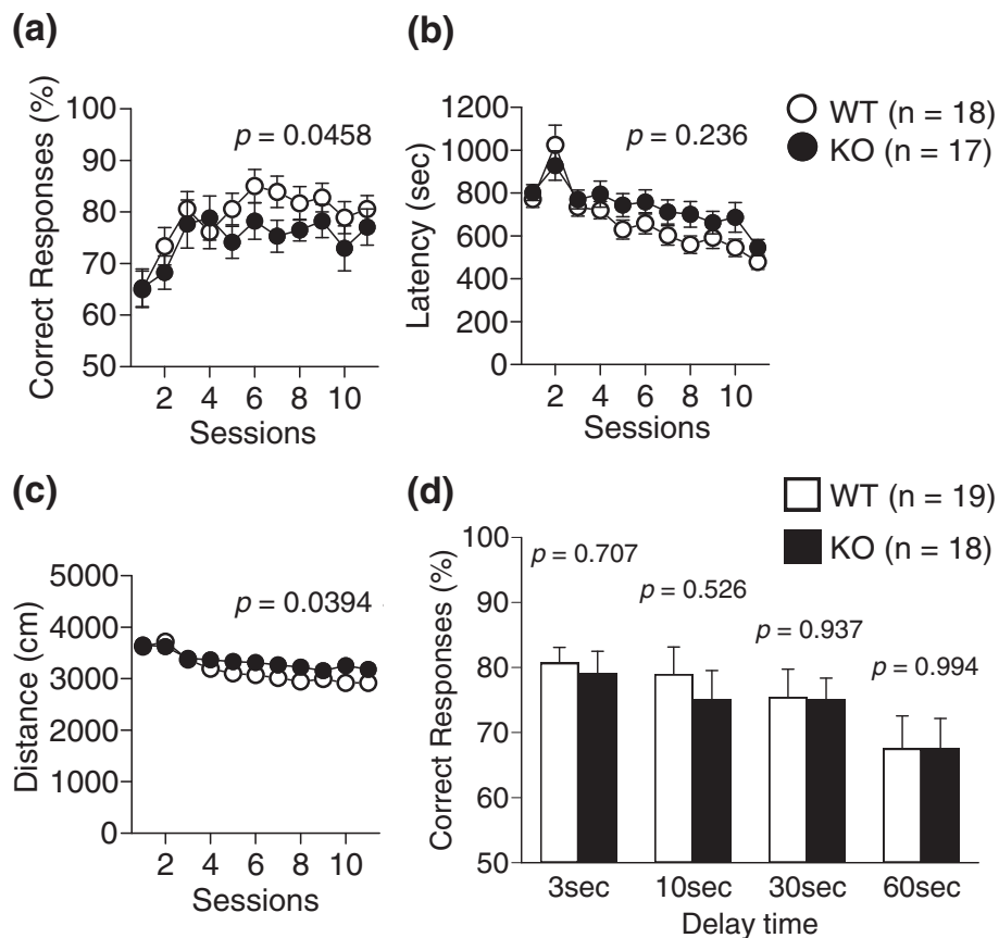
Figure 4 T-maze forced alternation task test. Correct response (a), latency (b), total distance (c), and correct response at various latency times (d) were recorded. The p -values indicate a genotype effect in the two-way repeated measures ANOVA (a-c) or Student's t -test (d). Data are given as mean ( \pm SEM).
