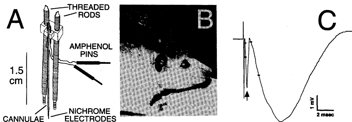
Fig. 1: A. Schematic of the implanted microdrive. A pair of 30 gauge cannulae, each containing a nichrome stimulating or recording electrode, is glued to an amphenol strip. The amphenol strip is loaded with two threaded stainless-steel support rods whose legs have been filed down to remove the threads. Grooves are then cut in the legs, allowing the influx of dental acrylic that prevents the legs from moving vertically after the drive is implanted. B. Photograph of a rat with the microdrive apparatus. The animal is shown connected to preamplifying headstage and recording and stimulating cable. C. Example of the Schaffer collateral evoked response, consisting of the presynaptic fiber potential ( \uparrow ) and the extracellular field EPSP. The cursors indicate the positions at which the fiber potential and the EPSP amplitudes were measured.
