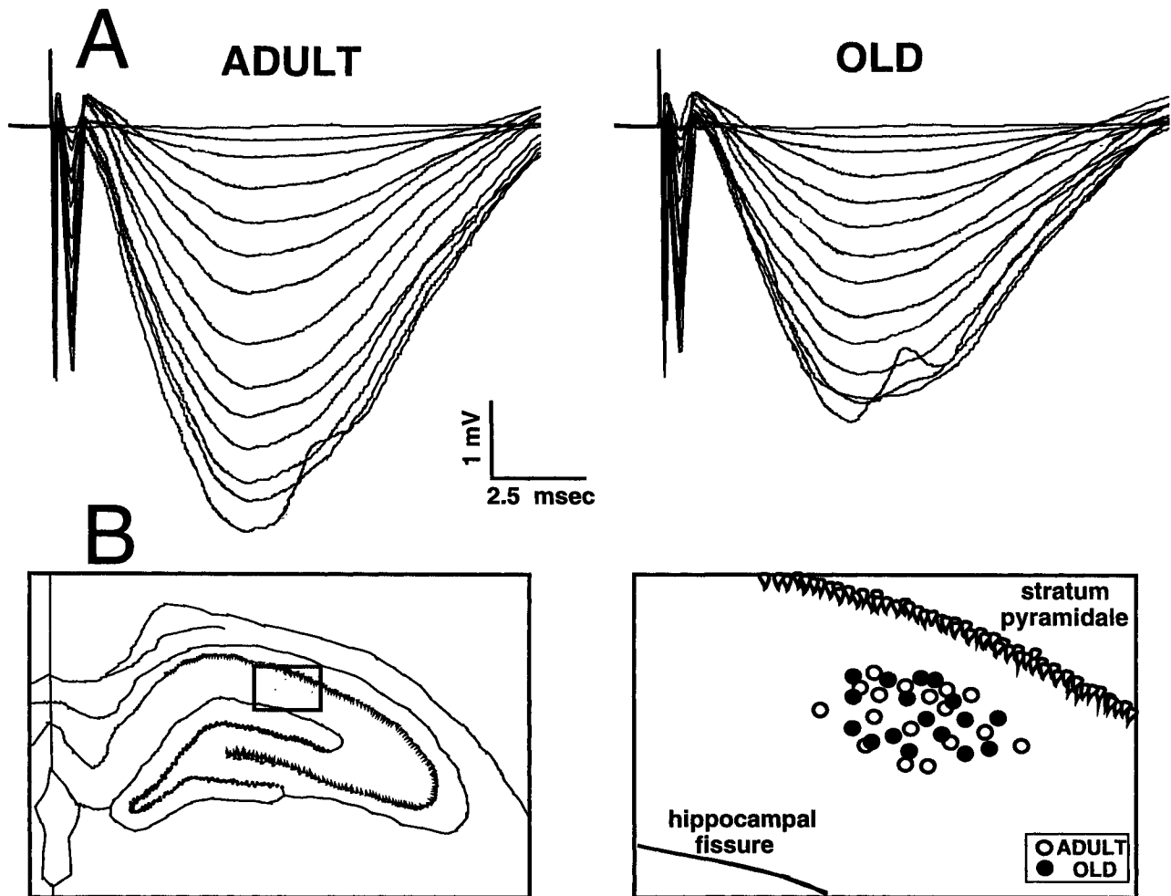
Fig. 3: A. Example of Schaffer collateral-CA1 pyramidal cell responses in one young and one old rat, collected at 14 different stimulus intensities. Each trace is an average of five individual evoked responses. B. Schematic diagram indicating the approximate locations of the recording sites at which the input-output series was conducted in CA1 stratum radiatum (○, adult; ● old).
