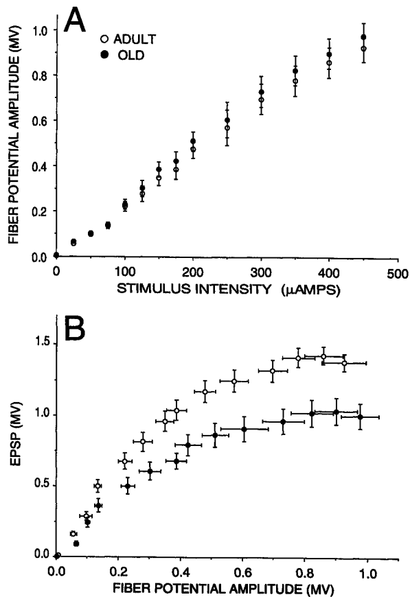
Fig. 4: Mean ( \pm SE) of the mean Schaffer collateral fiber potential amplitude, plotted for 14 stimulus levels (O, adult; n = 17 ; ● old, n = 17 ). B. Mean ( \pm SE) of the mean Schaffer collateral-CA1 evoked EPSP plotted relative to the mean fiber potential amplitude.
