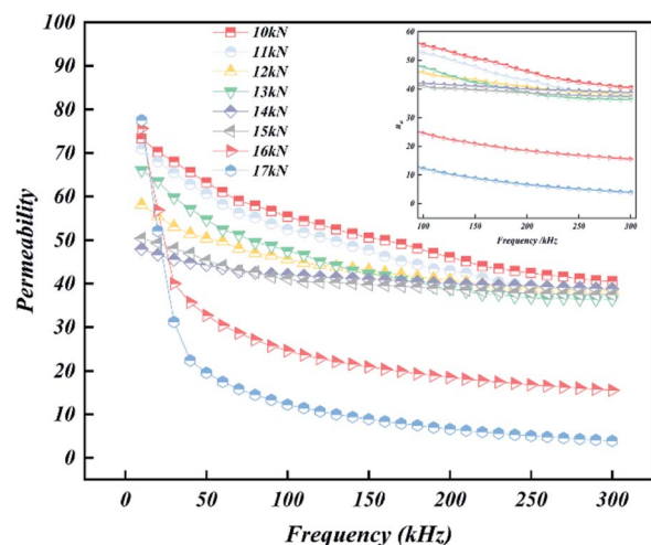
Fig. 5 Variation of the permeability of Fe-Si@SiO 2 SMPCs sintered at different axial pressures.
