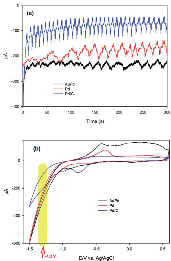
Fig. 4 (a) Chronoamperograms of AuPd, Pd and Pd/C at -1.3 V in PBS (pH 8.4), (b) cyclic voltammograms (CV) of AuPd, Pd and Pd/C in PBS (pH 8.4), scan rate: 50 mV s -1 .
