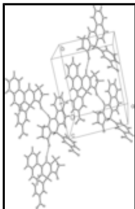
Fig. 2. The packing diagram of (I), Hydrogen bond represented by the dashed line.
