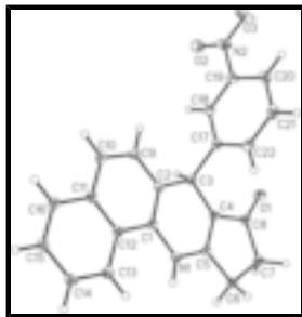
Fig. 1. The structure of (I), showing 30% probability displacement ellipsoids and the atom-numbering scheme. Cg is the centroid of the ring of C11/C12/C13/C14/C15/C16.
