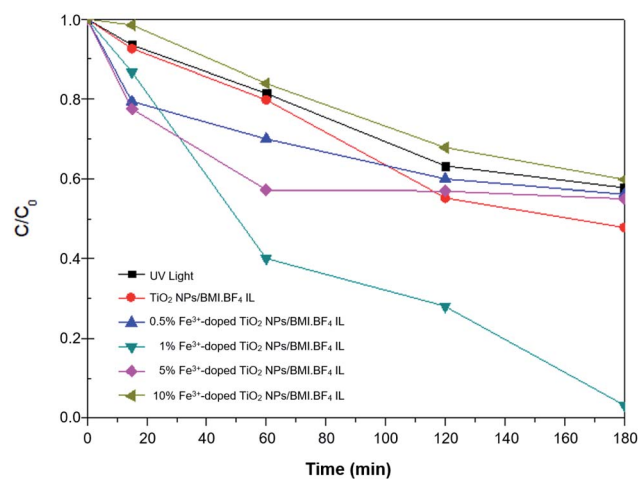
Fig. 11 Concentration versus time graph ( C/C_0 ) of the phenol photodegradation using the photocatalysts: UV light, TiO 2 NPs/BMI·BF 4 IL and 0.5; 1; 5 and 10%-doped Fe 3+ TiO 2 /BMI·BF 4 IL.
