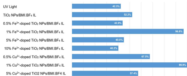
Fig. 10 Phenol photodegradation: (a) UV light, (b) TiO 2 NPs/BMI·BF 4 IL, (c) 0.5% Cu 2+ , (d) 1% Cu 2+ , (e) 5% Cu 2+ , (f) 0.5% Fe 3+ , (g) 1% Fe 3+ , (h) 5% Fe 3+ and (i) 10% Fe 3+ .
