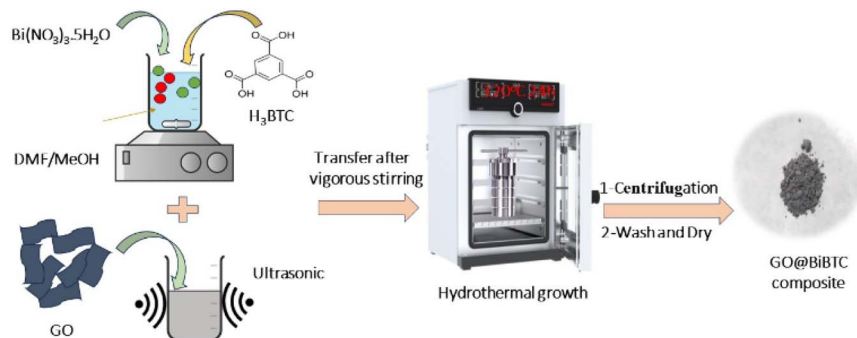
Scheme 1 The presentation of the synthesis of the GO@BiBTC MOF heterostructures.
