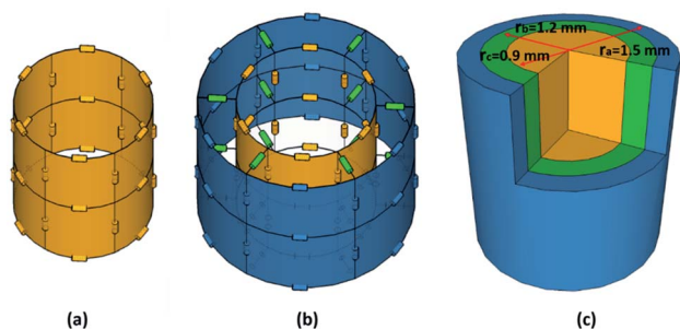
Fig. 8 The assumed structure of a CPC filament in this study. (a) A simple resistor network mimicking a filament with radially independent conductivity; (b) a resistor network with two concentric layers, connected radially with green resistors; (c) a resistor network with three concentric layers, where the radial resistors were omitted.
