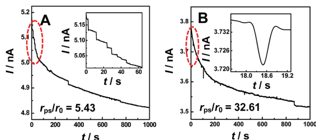
Fig. 1 Typical i - t traces obtained at nanopipets with a radius ( r_0 ) of 69 nm in 0.1 M KCl solution containing PS particles with different radii ( r_{ps} ). (A) r_{ps} = 375 nm, C_{ps} = 0.59 \mu\text{M} ; and (B) r_{ps} = 2.25 \mu\text{m} , C_{ps} = 16.9 \mu\text{M} . Insets: amplified current transients indicated with red circles in the figures. The applied potential was 200 mV. The data acquisition time was 10 ms.
