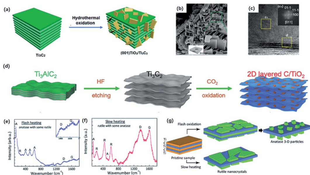
Fig. 6 (a) Schematic of the preparation of (001) \text{TiO}_2/\text{Ti}_3\text{C}_2 composite by hydrothermal treatment. (b) SEM photos of (001) \text{TiO}_2/\text{Ti}_3\text{C}_2 composite. (c) TEM image of (001) \text{TiO}_2/\text{Ti}_3\text{C}_2 . Inset (top-right) in (c): the indexed FFT image of \text{TiO}_2 showed the exposing (001) facets. 90 This figure has been reproduced from ref. 90 with permission from American Chemical Society, copyright 2016. (d) Scheme diagram of the preparation of 2D-layered C/ \text{TiO}_2 hybrids via \text{CO}_2 calcination. 82 This figure has been reproduced from ref. 82 with permission from Wiley-VCH, copyright 2017. (e, f) Raman spectra of the final product of flash heating and slow heating. 97 (g) Schematic diagram of two oxidation regimes including flash oxidation and slow heating. This figure has been reproduced from ref. 97 with permission from Royal Society of Chemistry, copyright 2014.
