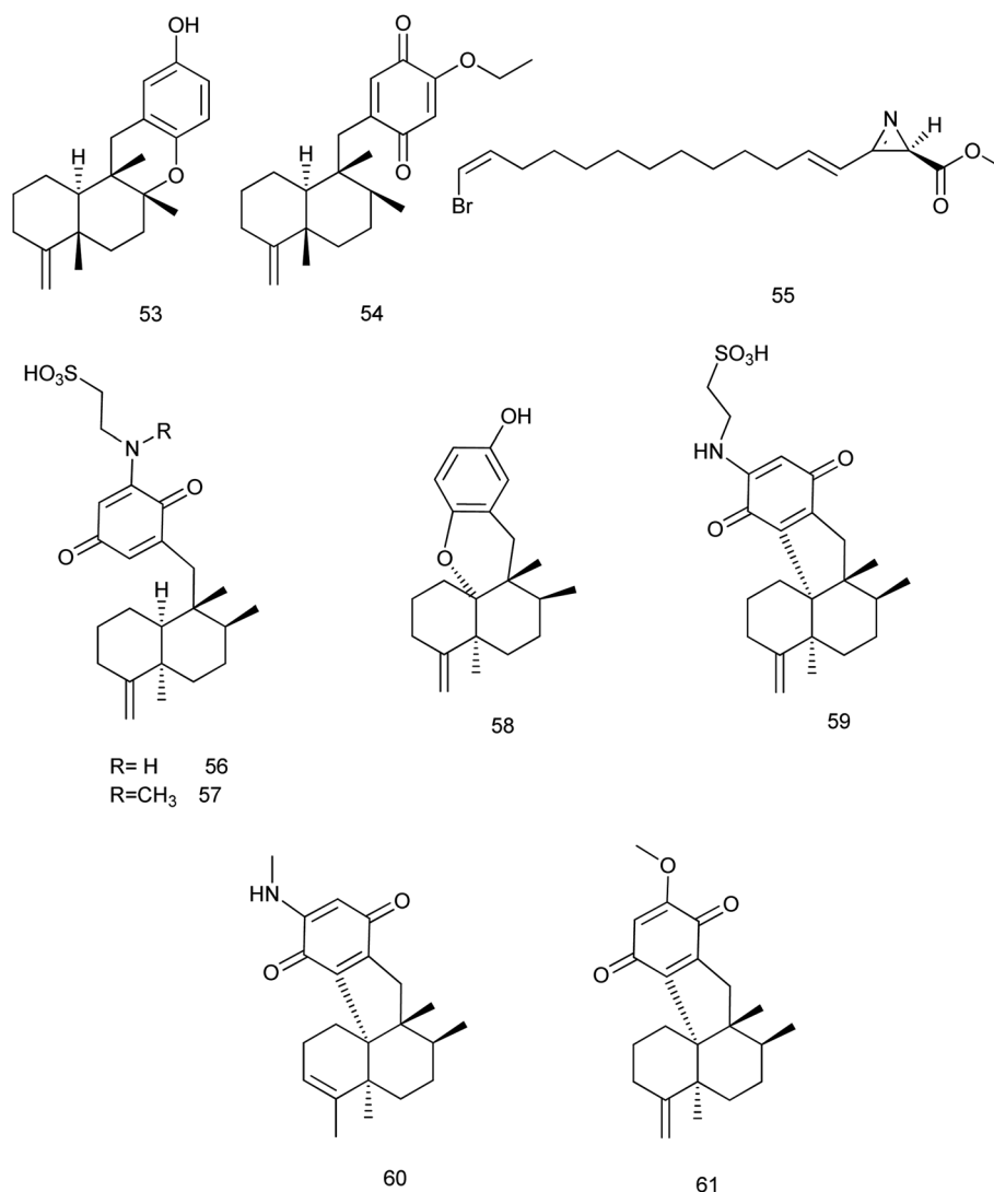
Fig. 6 Structures of compounds (53–61).
